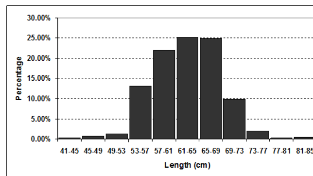
Figure 2: Percentage frequency of length E. affinis in Coastal Waters of Iran during 2003-05
