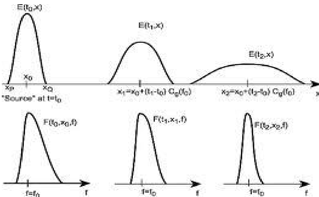
Figure 2.1: Distribution of swell waves in one dimension. At any given time the spectrum is given by a propagation of the spectra at t = t_0 .
